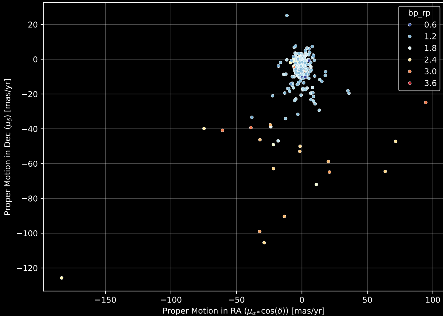
APOGEE DR17 Field: [K2_C7_010-10] Proper Motion Diagram (n= 278)
