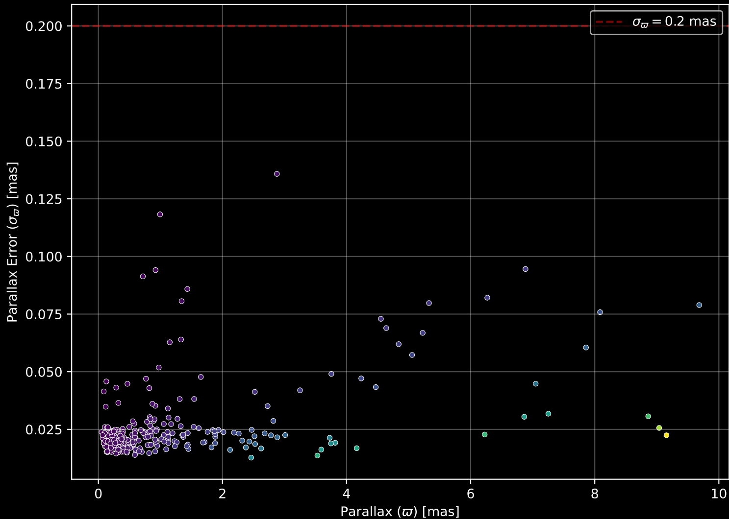
APOGEE DR17 Field: [K2_C7_010-10] Parallax Quality (n= 278)
