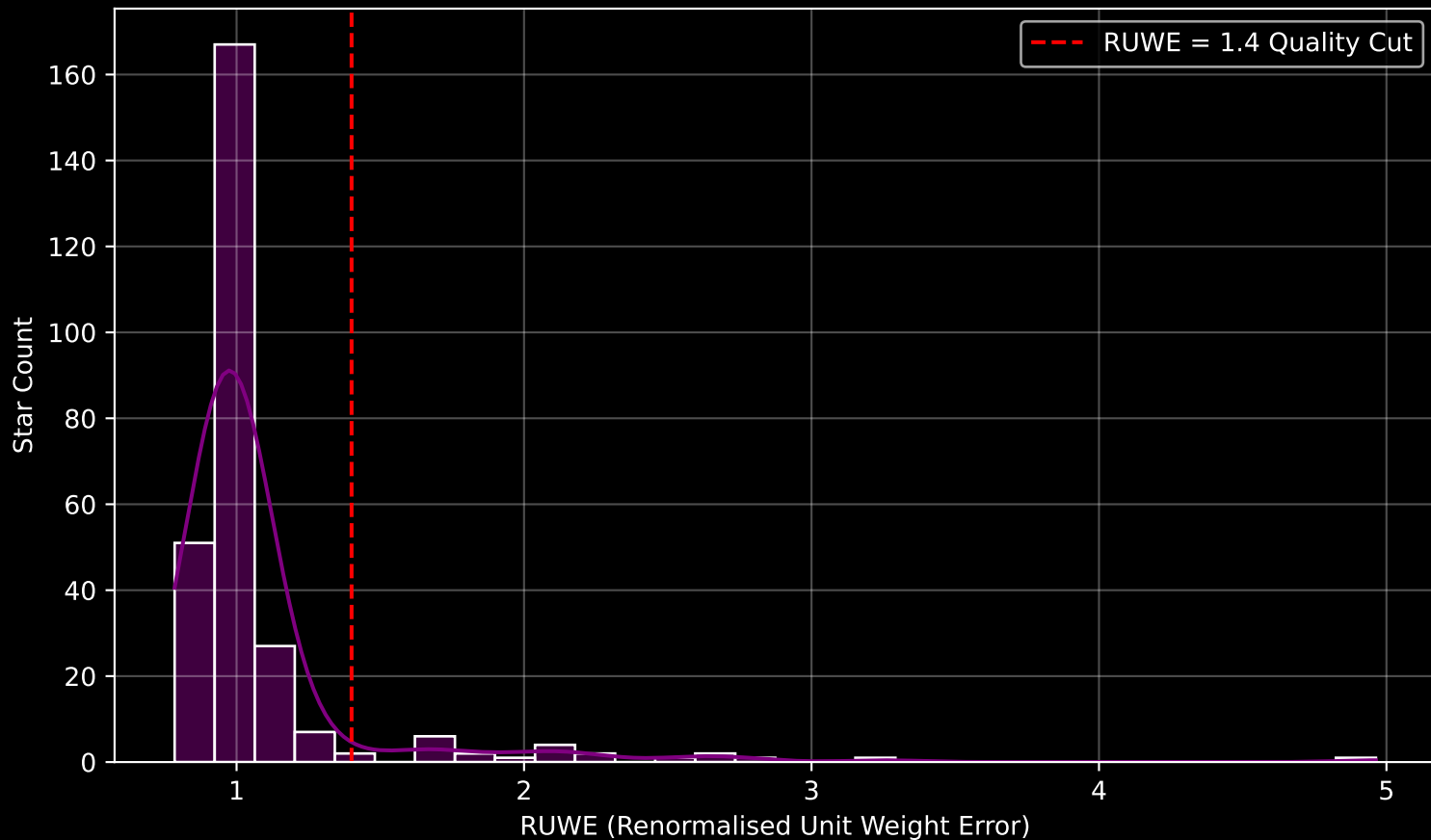
GAPOGEE DR17 Field [K2_C7_010-10] RUWE Distribution (n= 275)
