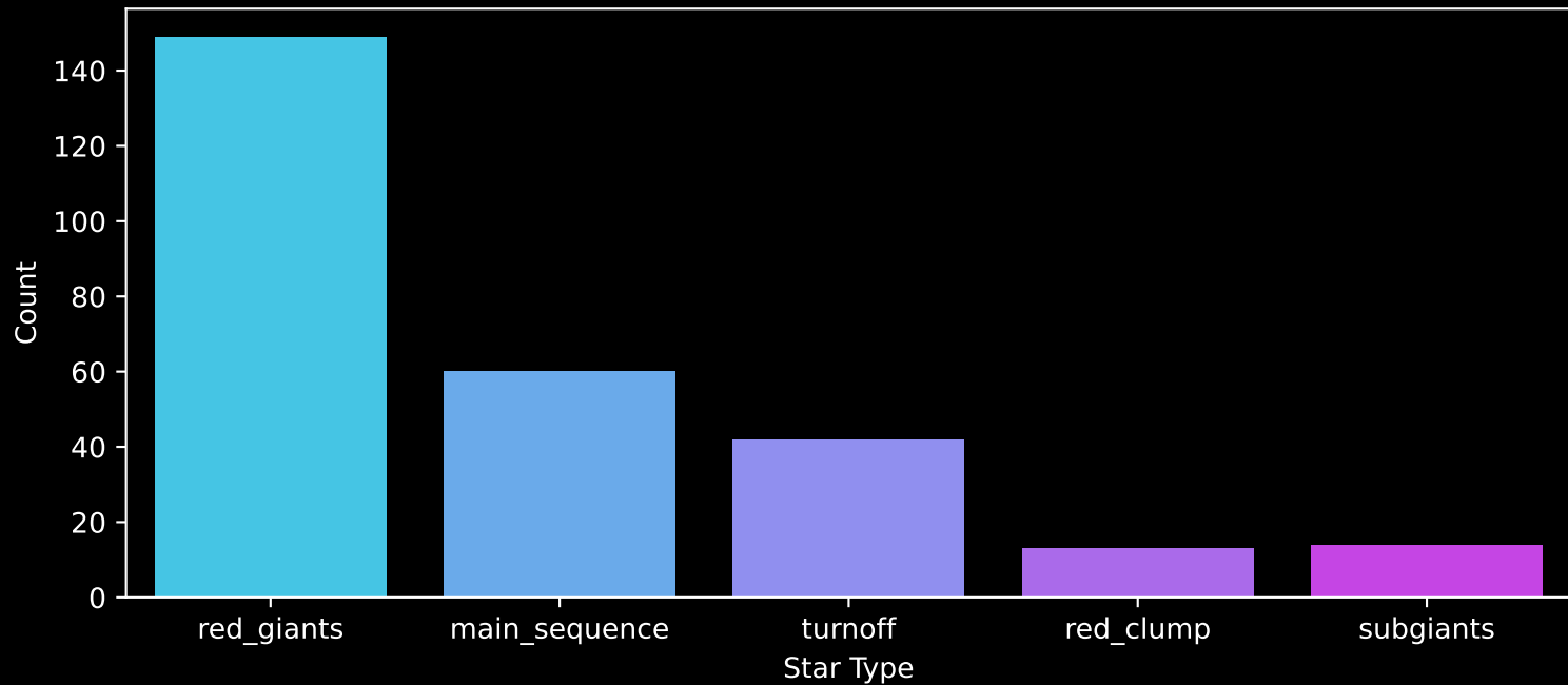
APOGEE DR17 Field: [K2_C7_010-10] Count plot of Star Type
