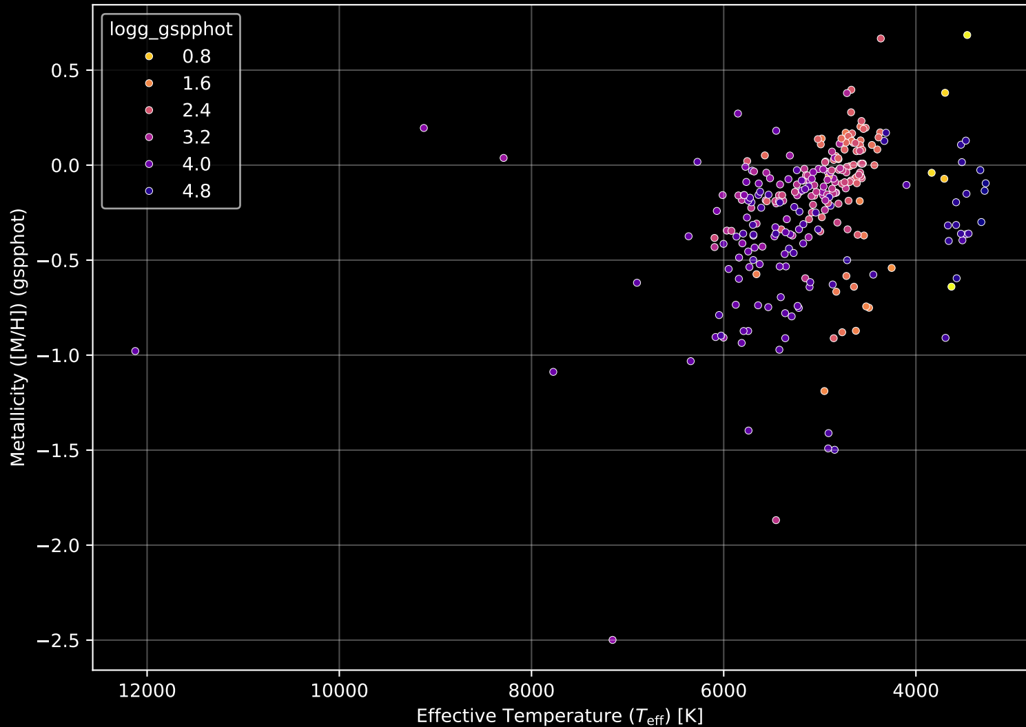
APOGEE DR17 Field: [K2_C7_010-10] Stellar Population Parameters (n= 278)
