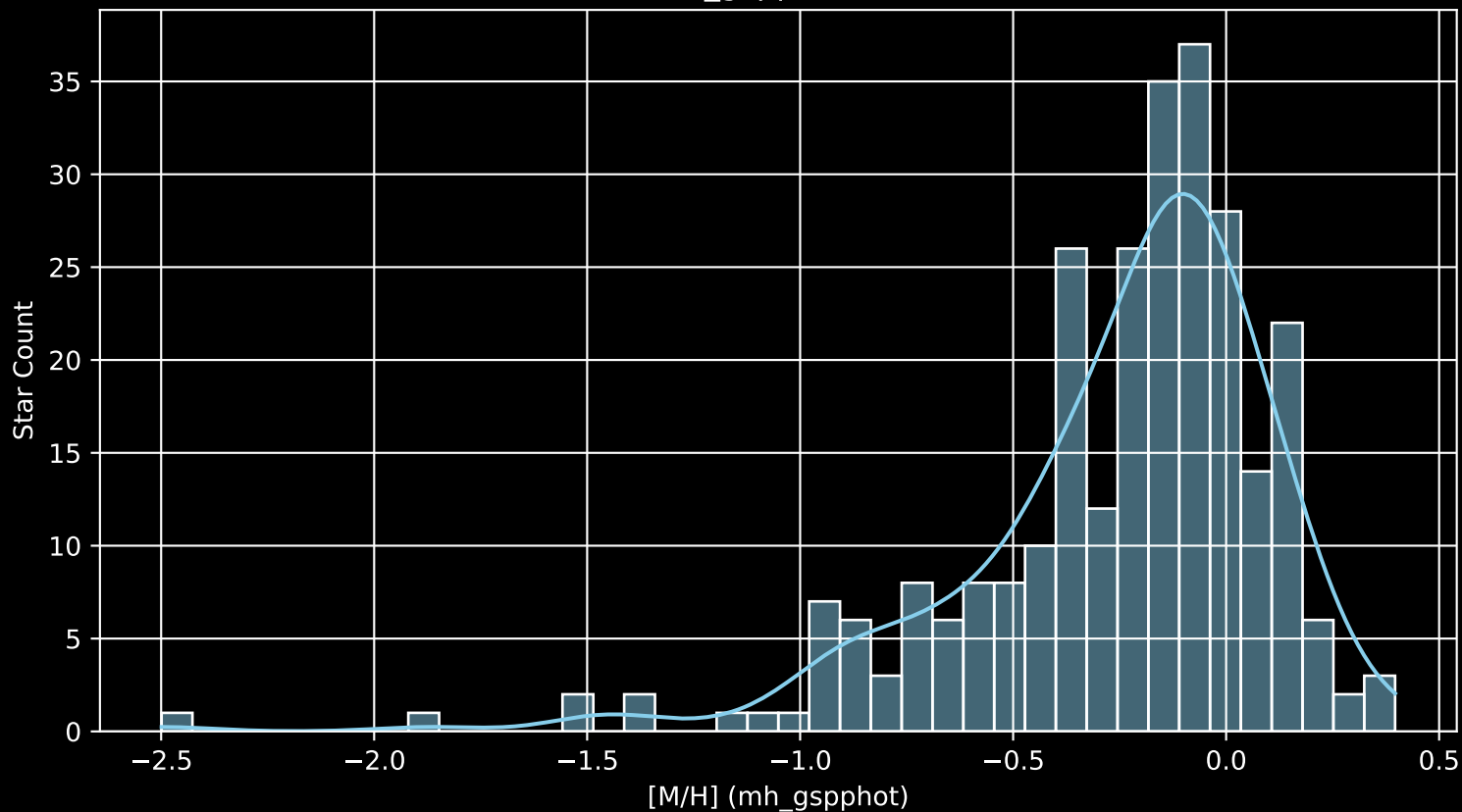
APOGEE DR17 Field: [K2_C7_010-10 [M/H] (mh_gspphot) (n= 276)
