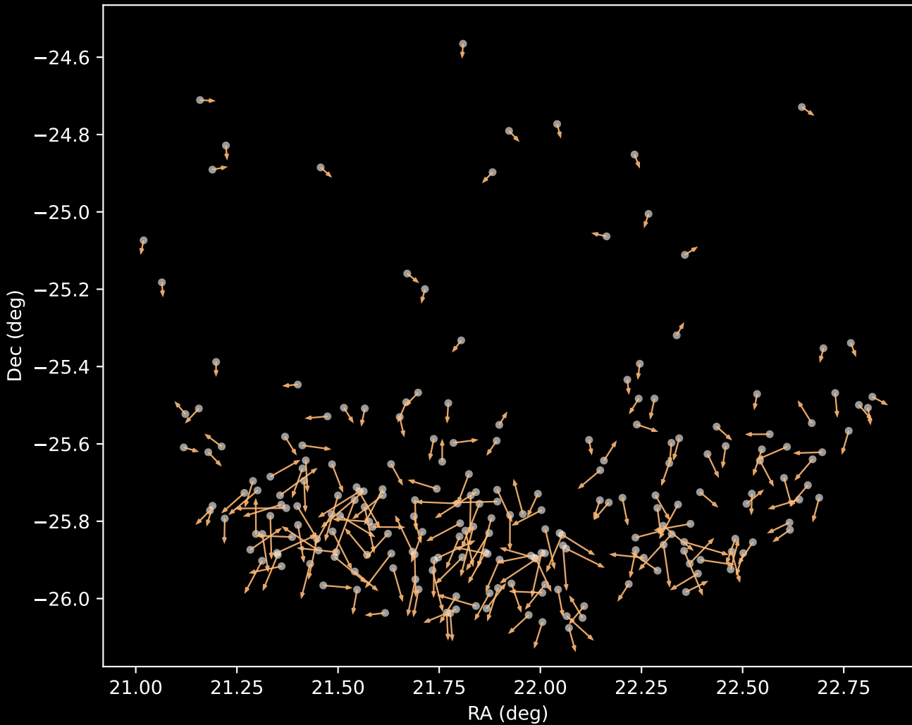
APOGEE DR17 Cluster 3 Proper Motion Vectors (n=216)
